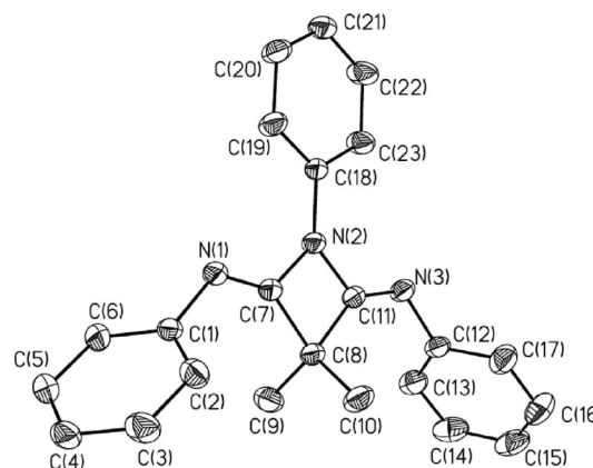
Figure 2. Molecular structure of 4 . Selected bond lengths [ \text{\AA} ] and bond angles [ ^\circ ]: N(1)–C(1) 1.424(3), N(3)–C(11) 1.261(3), N(1)–C(7) 1.251(3), N(2)–C(18) 1.418(3), N(2)–C(7) 1.409(3), N(3)–C(12) 1.420(3), N(2)–C(11) 1.403(3); N(1)–C(7)–N(2) 126.98(19), N(3)–C(11)–C(8) 140.9(2), N(1)–C(7)–C(8) 141.89(19), N(2)–C(11)–C(8) 91.93(16), N(2)–C(7)–C(8) 91.02(16), C(7)–N(1)–C(1) 121.99(19), C(7)–C(8)–C(11) 83.48(15), C(11)–N(3)–C(12) 121.1(2), N(3)–C(11)–N(2) 127.1(2). Hydrogen atoms on carbon atoms have been omitted for clarity.
