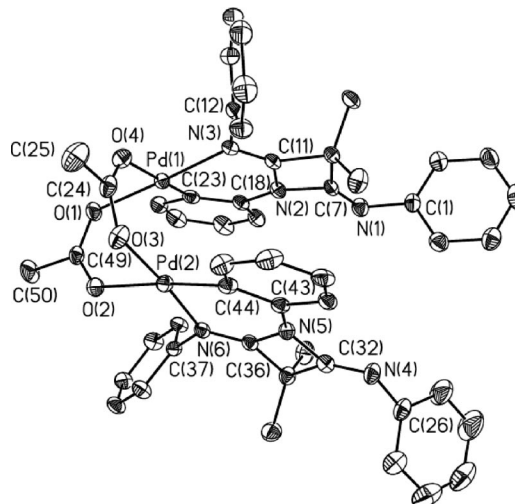
Figure 5. Molecular structure of 8 . Selected bond lengths [Å] and bond angles [°]: Pd(1)–Pd(2) 3.0818(8), Pd(1)–C(23) 1.988(4), Pd(2)–C(44) 2.004(4), Pd(1)–N(3) 2.030(3), Pd(2)–N(6) 2.021(3), Pd(1)–O(1) 2.041(3), Pd(2)–O(2) 2.131(3), Pd(1)–O(4) 2.126(3), Pd(2)–O(3) 2.042(3), C(18)–C(23) 1.387(5), C(43)–C(44) 1.394(5), C(18)–N(2) 1.427(5), C(43)–N(5) 1.422(5), N(3)–C(11) 1.274(5), N(6)–C(36) 1.268(5); C(23)–Pd(1)–N(3) 91.78(14), C(44)–Pd(2)–N(6) 92.71(14), C(23)–Pd(1)–O(1) 89.39(14), C(44)–Pd(2)–O(3) 89.94(14), N(3)–Pd(1)–O(1) 178.06(12), N(6)–Pd(2)–O(3) 175.68(13), C(23)–Pd(1)–O(4) 174.37(14), C(44)–Pd(2)–O(2) 172.49(14), N(3)–Pd(1)–O(4) 91.47(12), N(6)–Pd(2)–O(2) 90.16(11), O(1)–Pd(1)–O(4) 87.23(12), O(2)–Pd(2)–O(3) 86.81(12). Hydrogen atoms on carbon atoms have been omitted for clarity.
