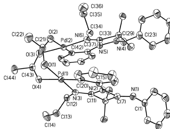
Figure 4. Molecular structure of 7 . Selected bond lengths [Å] and bond angles [°]: Pd(1)–Pd(2) 2.9409(4), Pd(1)–C(20) 1.995(3), Pd(2)–C(42) 2.002(3), Pd(1)–N(3) 2.015(3), Pd(2)–N(6) 2.024(3), Pd(1)–O(1) 2.048(2), Pd(2)–O(2) 2.158(2), Pd(1)–O(4) 2.142(2), Pd(2)–O(3) 2.048(2), C(15)–C(20) 1.389(4), C(42)–C(37) 1.402(4), C(15)–N(2) 1.415(4), C(37)–N(5) 1.415(4), N(3)–C(11) 1.258(4), N(6)–C(33) 1.265(4); C(20)–Pd(1)–N(3) 93.10(11), C(42)–Pd(2)–N(6) 93.76(11), C(20)–Pd(1)–O(1) 90.48(12), C(42)–Pd(2)–O(3) 91.41(12), N(3)–Pd(1)–O(1) 176.31(10), N(6)–Pd(2)–O(3) 174.45(10), C(20)–Pd(1)–O(4) 173.24(11), C(42)–Pd(2)–O(2) 172.04(11), N(3)–Pd(1)–O(4) 92.32(10), N(6)–Pd(2)–O(2) 92.17(10), O(1)–Pd(1)–O(4) 84.17(11), O(3)–Pd(2)–O(2) 82.50(11). Hydrogen atoms on carbon atoms have been omitted for clarity.
